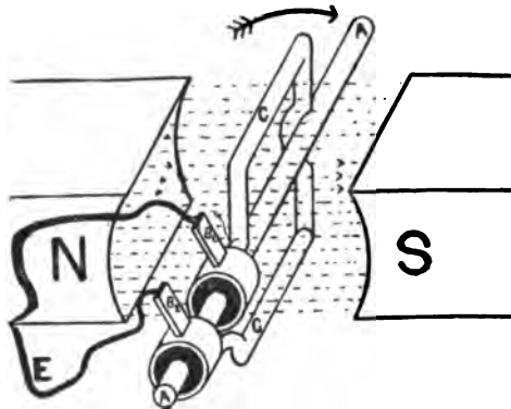
FIG. 427.—Diagram of a Dynamo Electrical Generator, arranged for producing an alternating current, showing the constructional and operative features. Here N and S are the positive and negative poles of the field magnets, between which the lines of force are shown by the dotted lines. A is the armature spindle; B 1 and B 2 , the brushes bearing on the ring drums; C, the coil, or winding, of the armature; E, the outside circuit to which the current is supplied.
